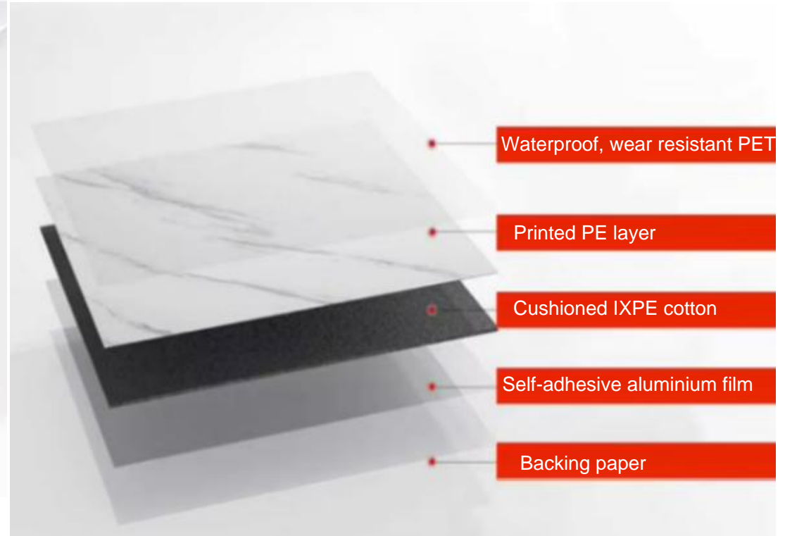
Backing paper Aluminium plating film Foam layer Printed layer
